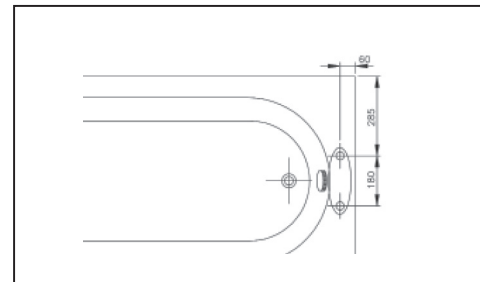
Bath Filler one Hole / Tek Delikli Batarya
