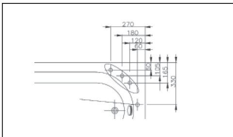
Bath Filler 2 Holes / İki Delikli Batarya
