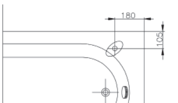
Bath Filler 2 Holes / İki Delikli Batarya
